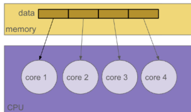
Figure 1.9.1: Data parallelism is when data is divided among processors to perform the same task to each subset.
